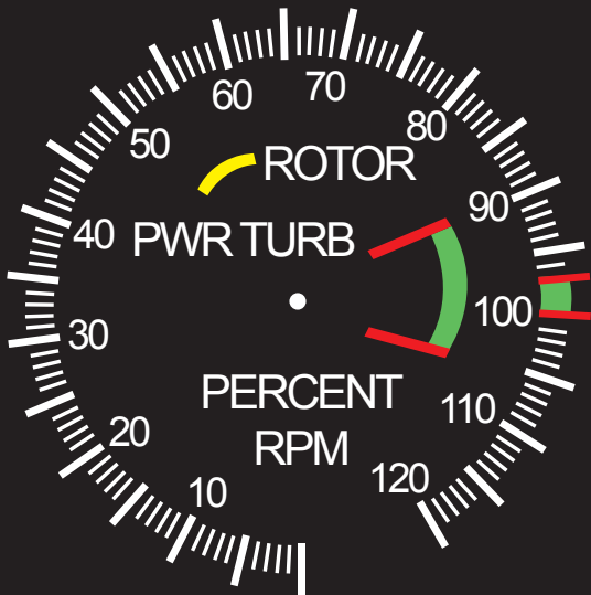
Bell206 rotor/turbine % RPM
